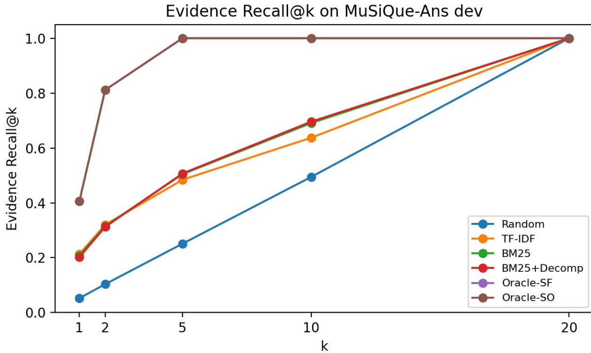
Figure 4. Evidence Recall@k curves for different retrievers and oracles on MuSiQue-Ans dev.
