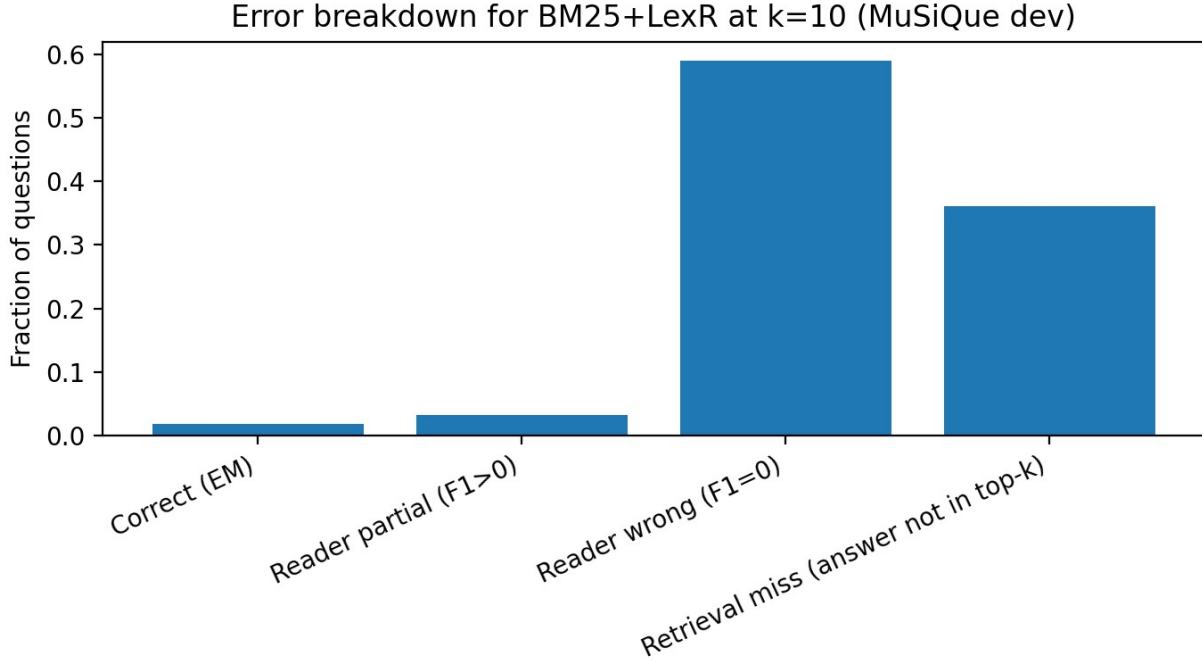
Figure 6. Error breakdown fractions for BM25+LexR at k=10 (same categories as Table 11).
