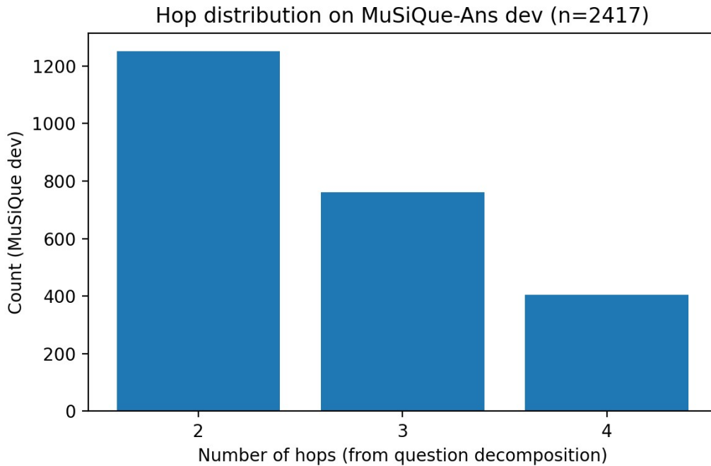
Figure 2. Hop distribution derived from MuSiQue gold decompositions (2-hop/3-hop/4-hop).
