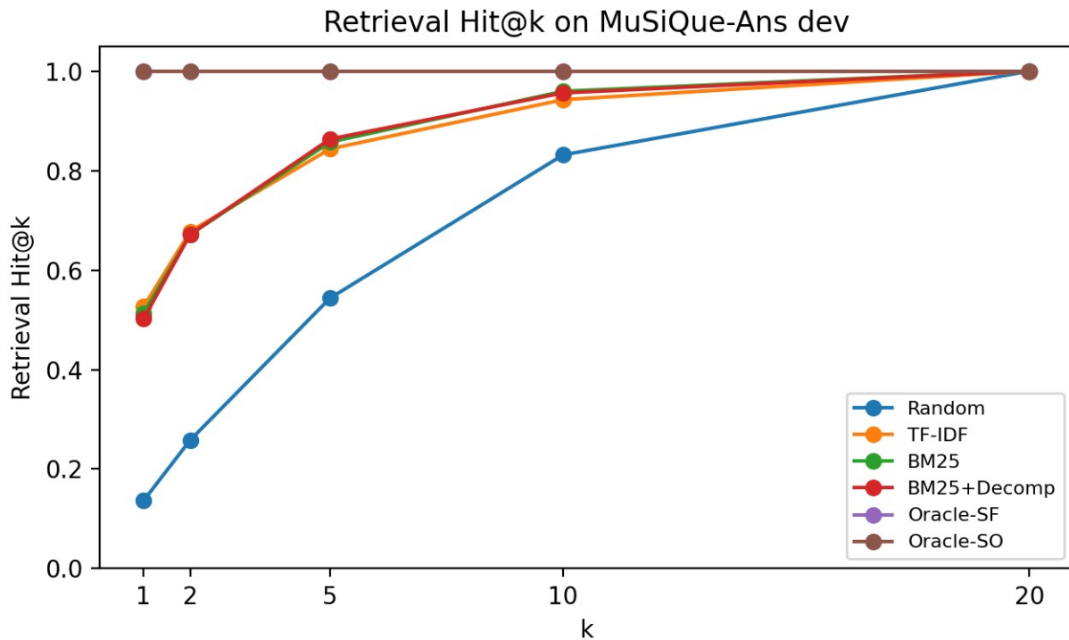
Figure 3. Retrieval Hit@ k curves for different retrievers and oracles on MuSiQue-Ans dev.
