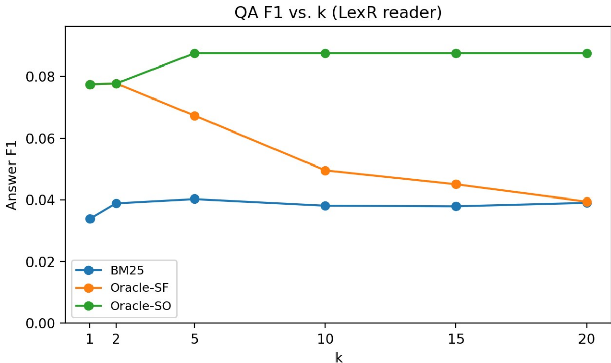
Figure 5. QA F1 vs. k for BM25 and oracle retrieval variants (LexR reader).
