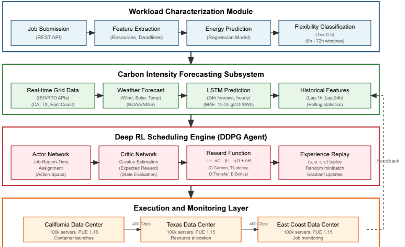
Figure 1: CarbonShift Framework Architecture
