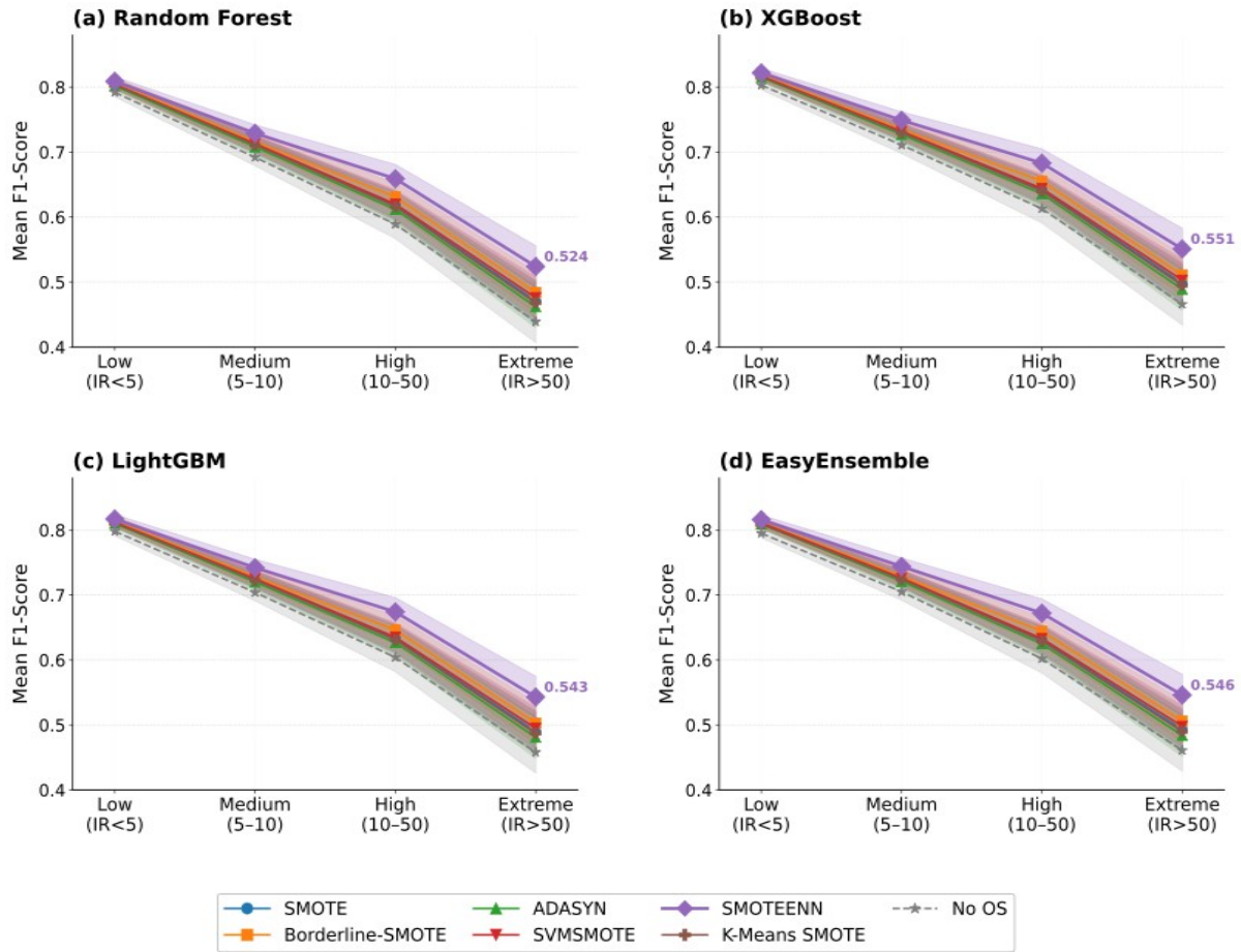
Figure 2: Effect of Imbalance Ratio on F1-Score Across Oversampling Methods and Ensemble Classifiers
