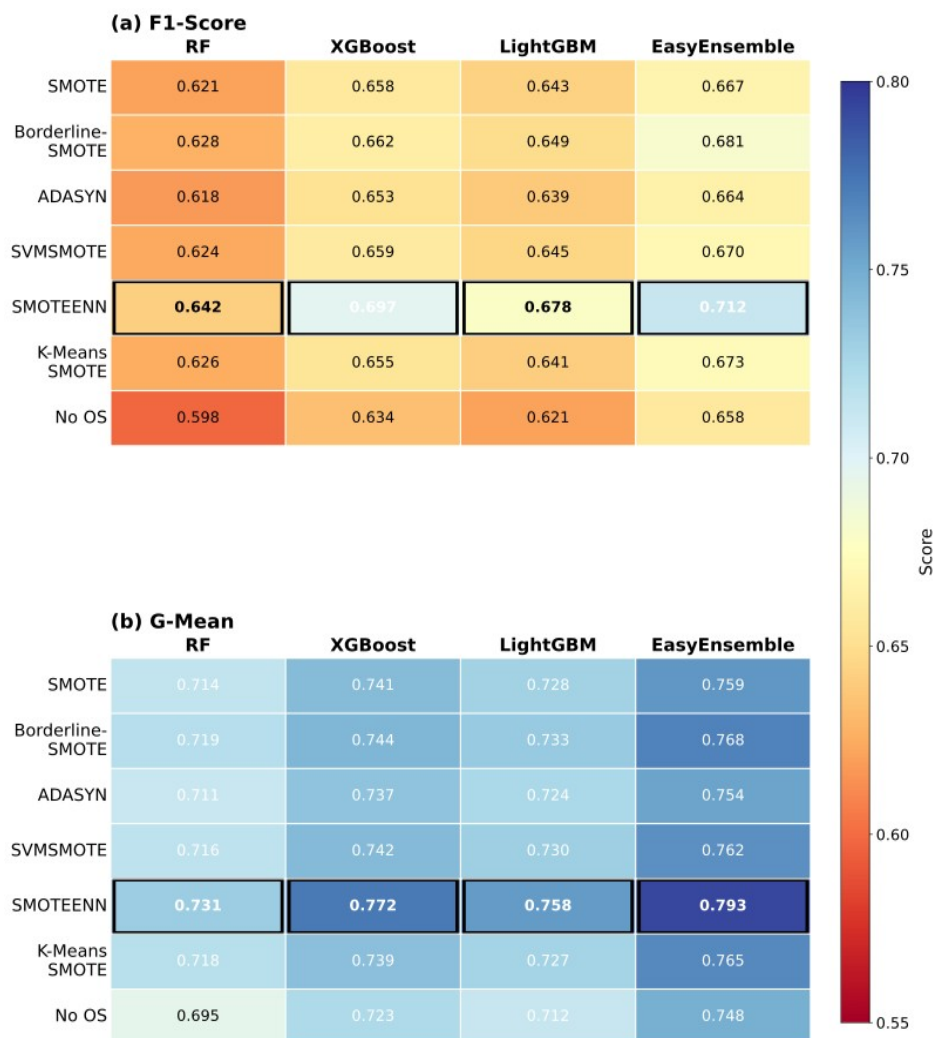
Figure 1: Mean F1-Score and G-Mean Heatmap Across All Oversampling-Ensemble Combinations
