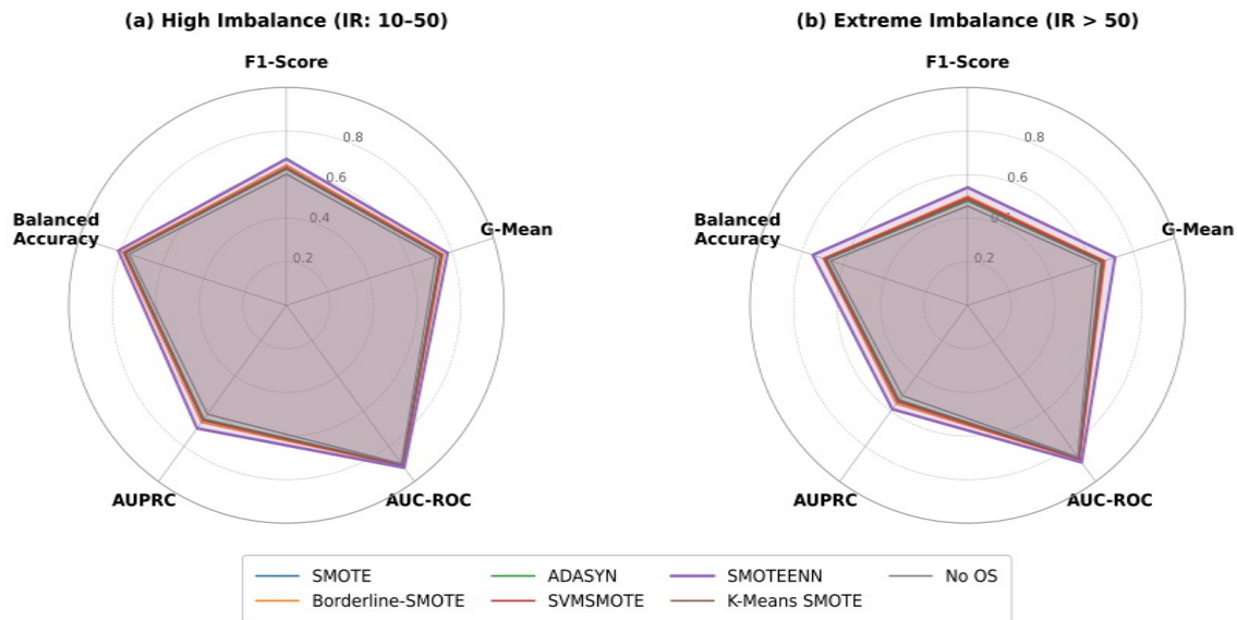
Figure 3 description. A side-by-side pair of radar (spider) charts generated using matplotlib's polar projection, displayed at 14 \times 7 inches at 300 dpi. The left panel presents results for the High IR group (IR 10–50) and the right panel presents results for the Extreme IR group (IR > 50). Each radar chart has five axes arranged at 72-degree intervals, corresponding to five performance metrics: F1-score, G-mean, AUC-ROC, AUPRC, and Balanced Accuracy. The radial scale on all axes runs from 0.0 (center) to 1.0 (outer ring), with concentric gridlines at 0.2, 0.4, 0.6, and 0.8 drawn as thin dashed gray circles. Metric labels are positioned 0.15 units beyond the outer ring along each axis direction. Seven filled polygons—one per oversampling configuration including the no-oversampling baseline—are superimposed using a tab10 color palette. Each polygon uses a semi-transparent fill ( \alpha = 0.15 ) and a solid boundary line (linewidth = 1.8). The SMOTEENN polygon uses linewidth = 2.5 and a slightly higher alpha (0.25) to distinguish it visually. A shared legend listing all seven configurations is positioned to the right of the right panel. Axis tick values are hidden to reduce clutter; only the gridline values (0.2, 0.4, 0.6, 0.8) are annotated in small gray text (fontsize = 8). The two panel titles read "High Imbalance (IR: 10–50)" and "Extreme Imbalance (IR > 50)" respectively in bold fontsize 12. The overall figure title reads "Performance Profiles of Oversampling Methods with EasyEnsemble: High vs. Extreme Imbalance."
