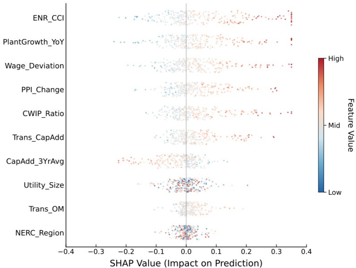
Figure 2. SHAP Summary Plot for the Top Ten Features in the LightGBM Classifier
