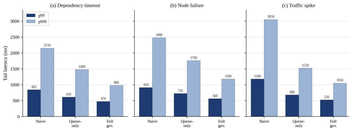
Figure 2. Tail Latency Across Three Configurations and Three Fault Classes
