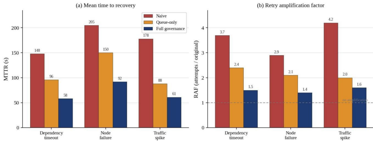
Figure 3. Recovery Time and Retry Amplification by Fault Class
