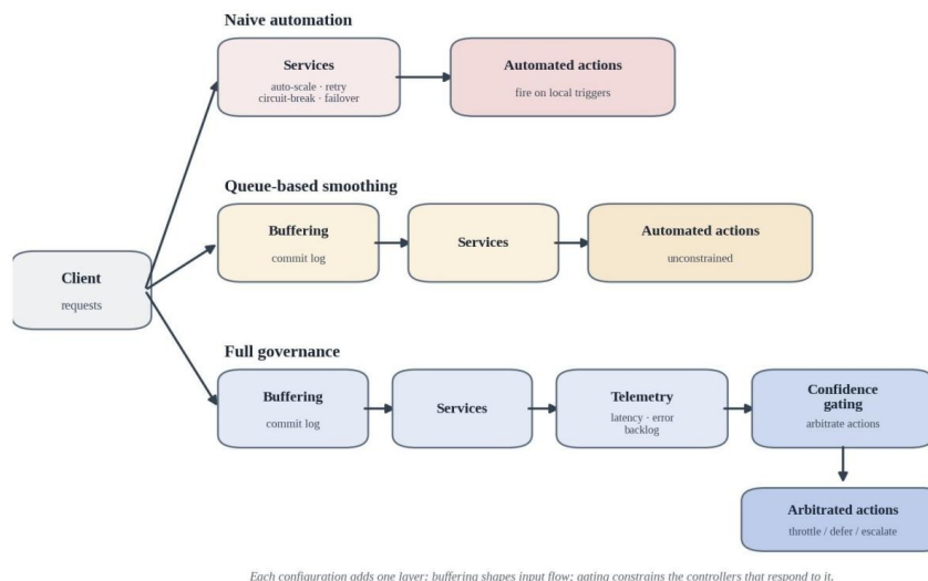
Figure 1. Experimental Configurations and the Closed-Loop Arbitration Path
