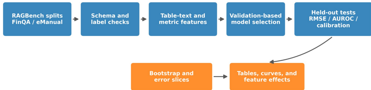
Figure 1. Experimental workflow for table-text RAG answer-quality regression.
