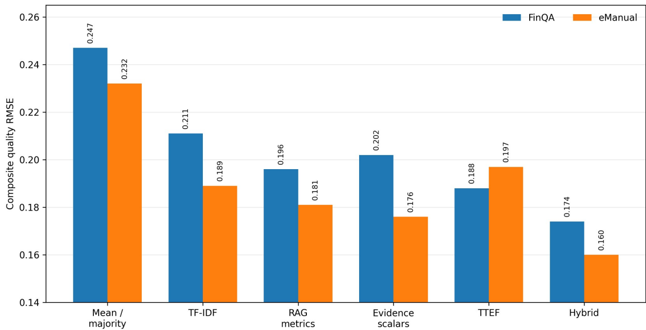
Figure 4. Test-set composite quality RMSE by model family and dataset.
