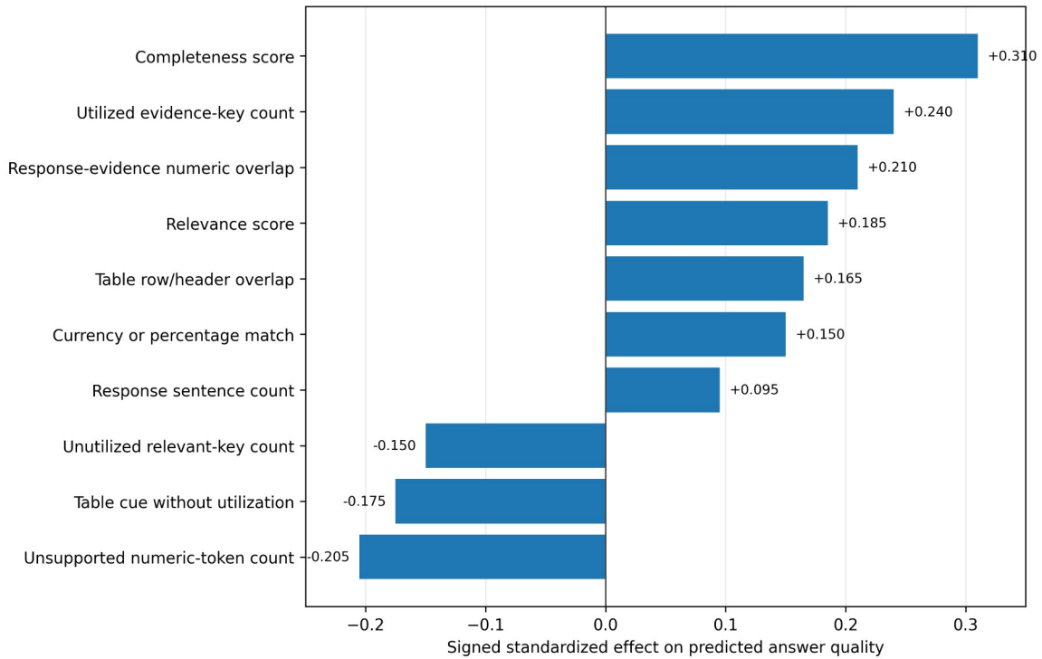
Figure 5. Signed standardized feature effects in the FinQA hybrid model.
