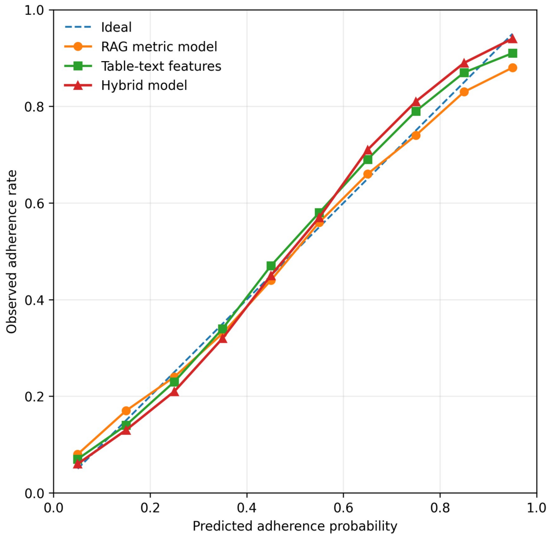
Figure 6. FinQA adherence calibration by model family.
