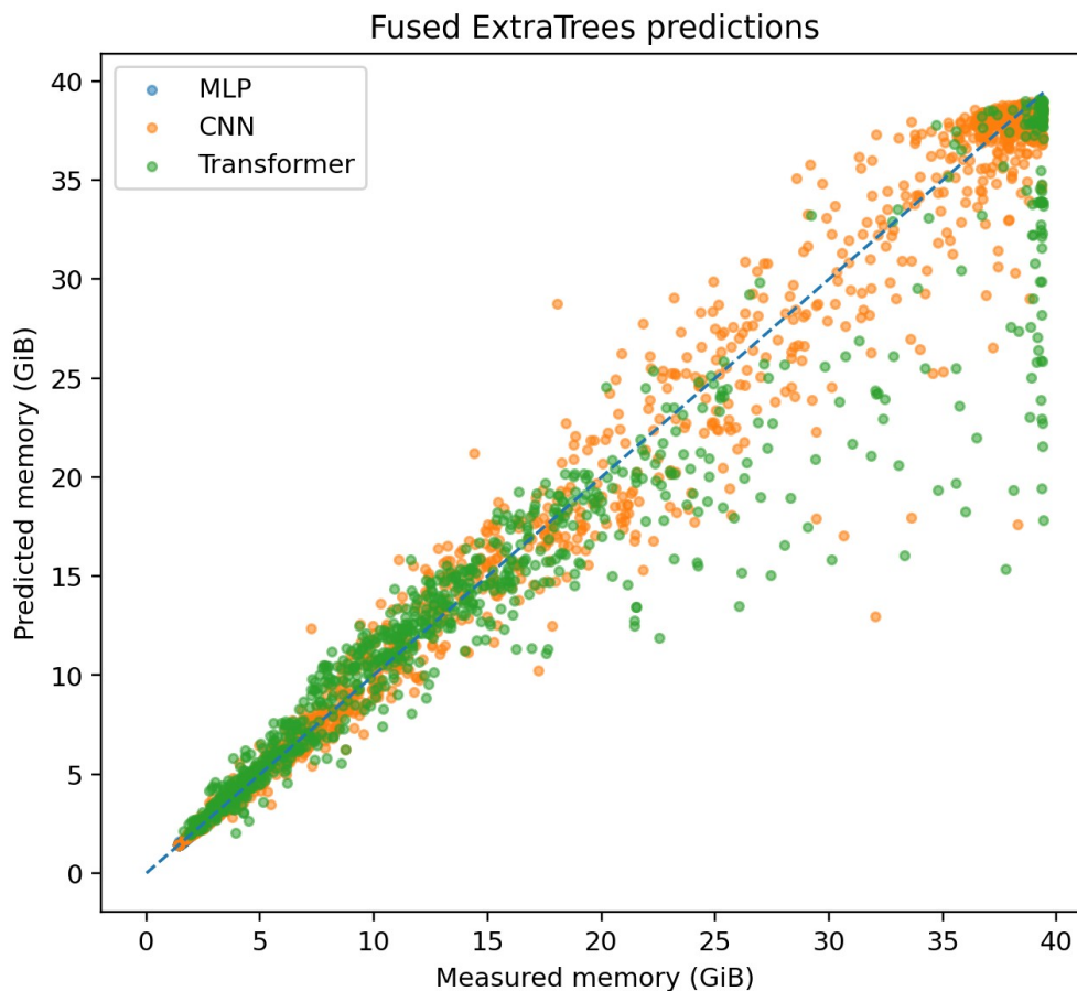
Figure 4. Fused ExtraTrees predictions versus measured memory on the mixed test split.
