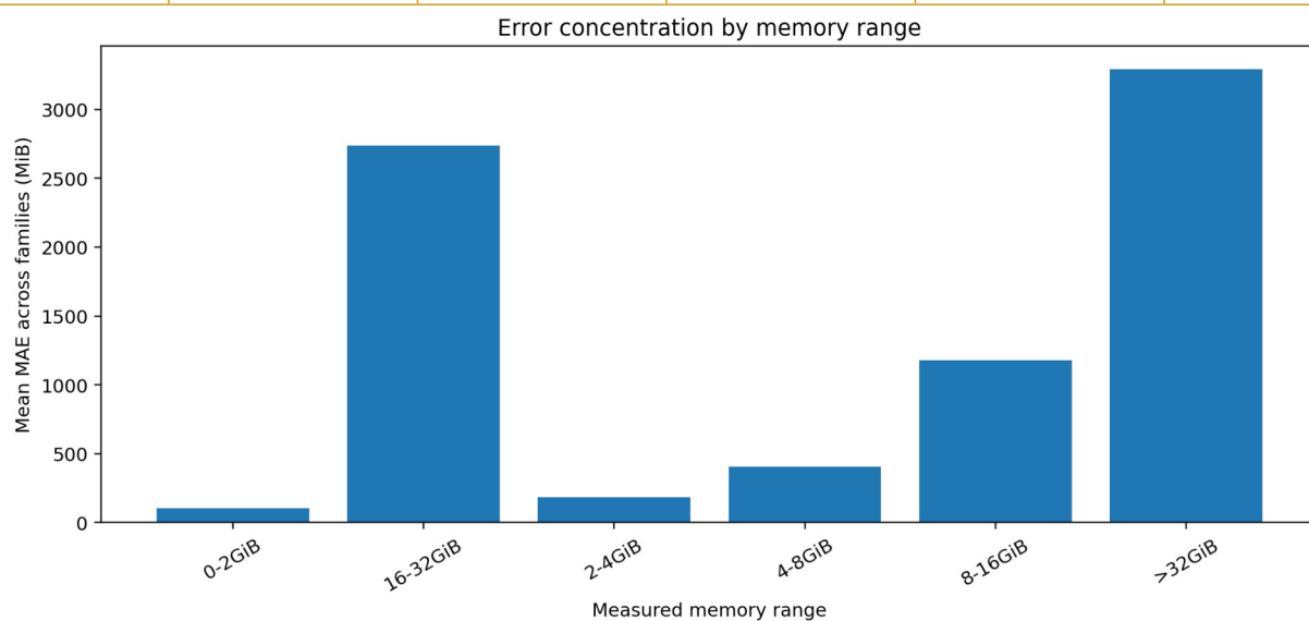
Figure 7. Mean absolute error by measured memory range.
