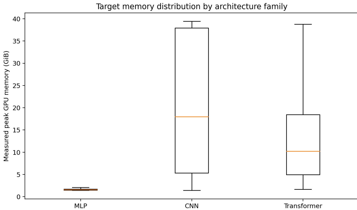
Figure 2. Distribution of measured peak GPU memory by architecture family.
