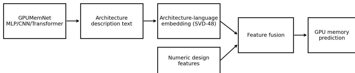
Figure 1. End-to-end architecture-description and numeric-feature fusion pipeline.
