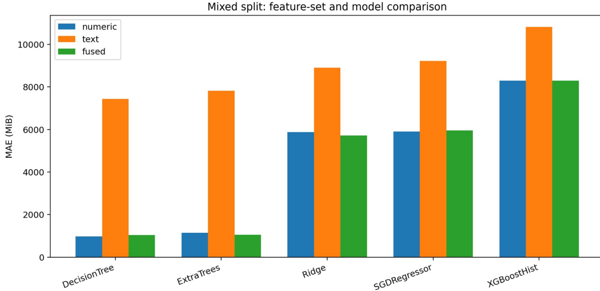
Figure 3. Mixed-split comparison of feature sets and supervised regressors.
