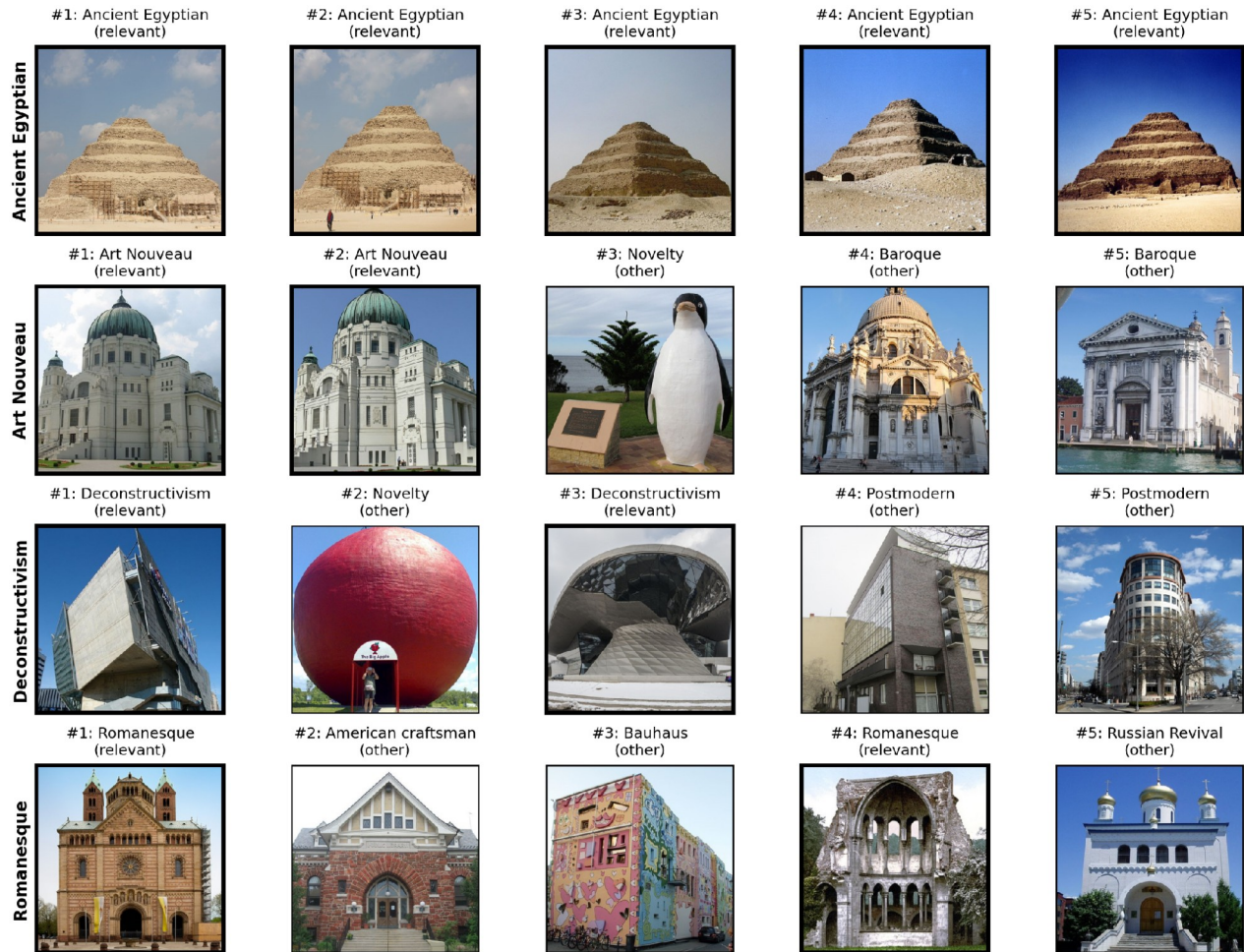
Figure 5. Top-five text-to-image results for four style queries using calibrated hybrid scores. Heavy borders mark relevant images, and titles state the manifest class.
