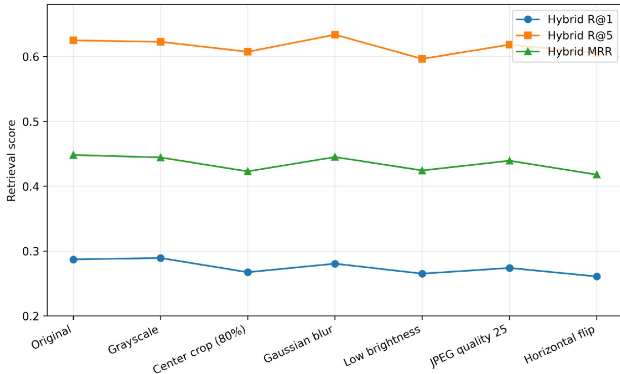
Figure 9. Hybrid retrieval under six held-out image perturbations. Models and transformations were fitted on original training images only.
