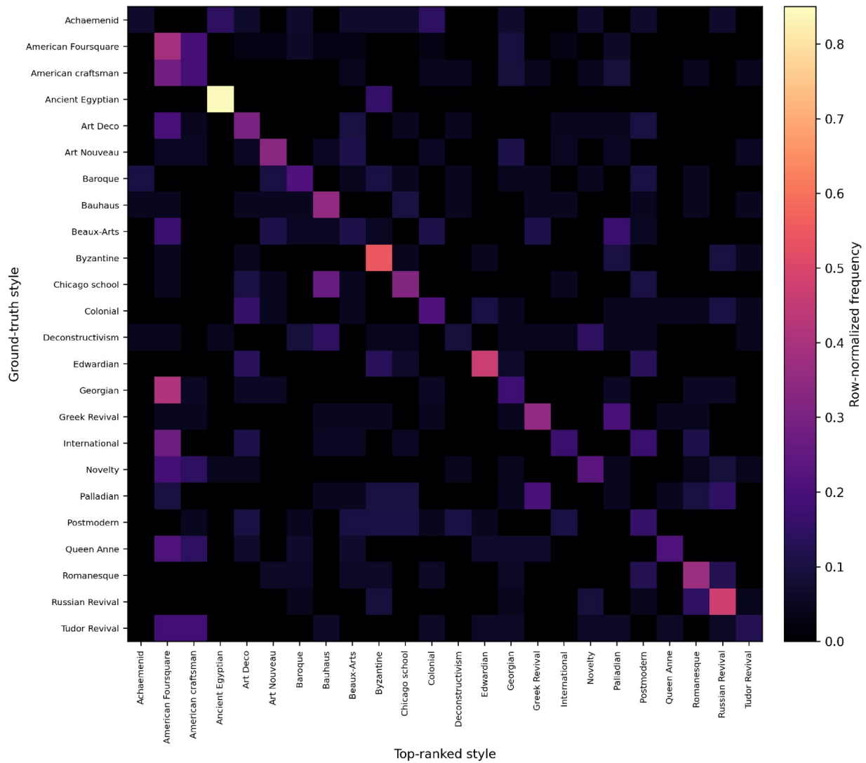
Figure 8. Row-normalized top-rank confusion matrix for the PGAR calibrated hybrid. Bright diagonal cells indicate high per-style Recall@1.
