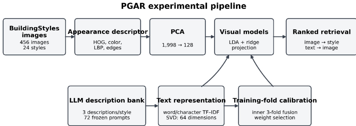
Figure 1. PGAR experimental pipeline. Image transforms were fitted inside each outer training fold; the language bank was generated once and then held fixed.
