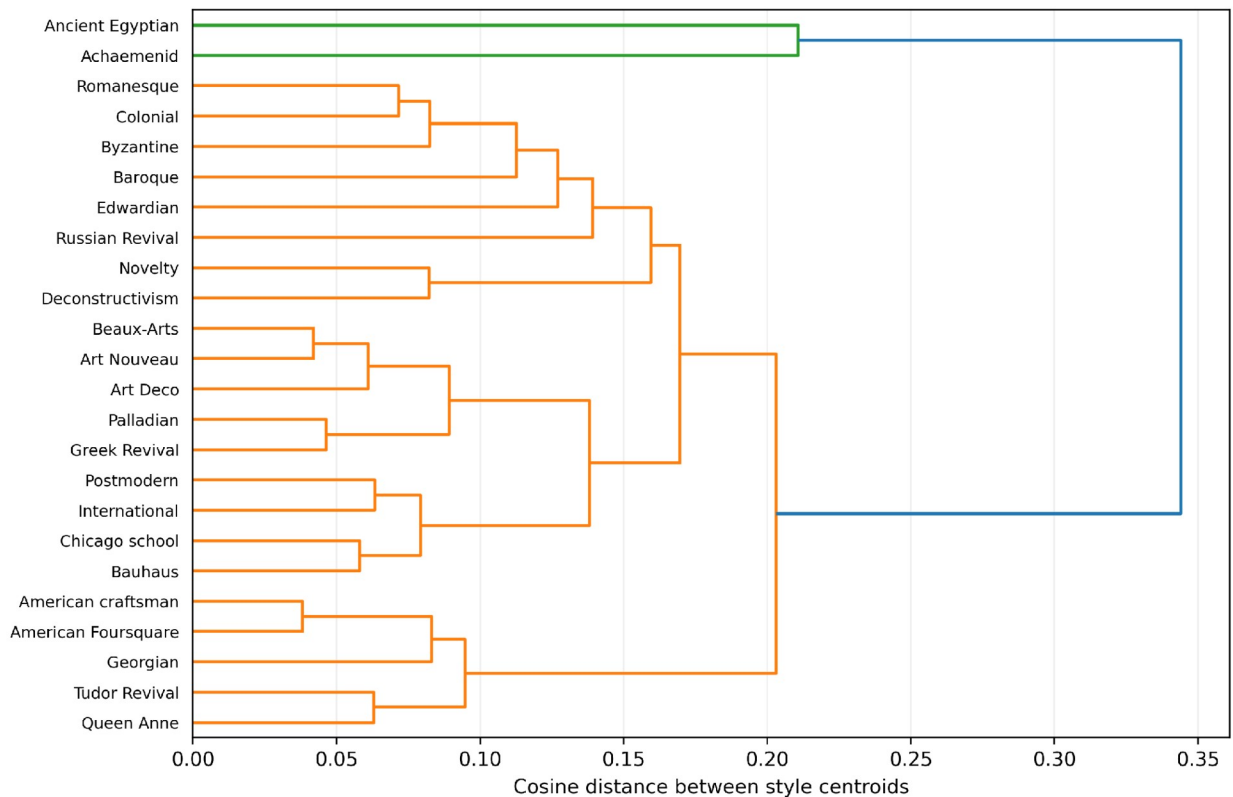
Figure 7. Average-linkage clustering of normalized style centroids using cosine distance. Short branches identify styles with similar held-out prompt projections.
