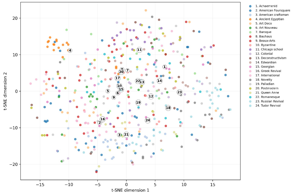
Figure 6. t-SNE visualization of the 64-dimensional held-out prompt projections. Numeric labels mark class centroids and correspond to the legend.
