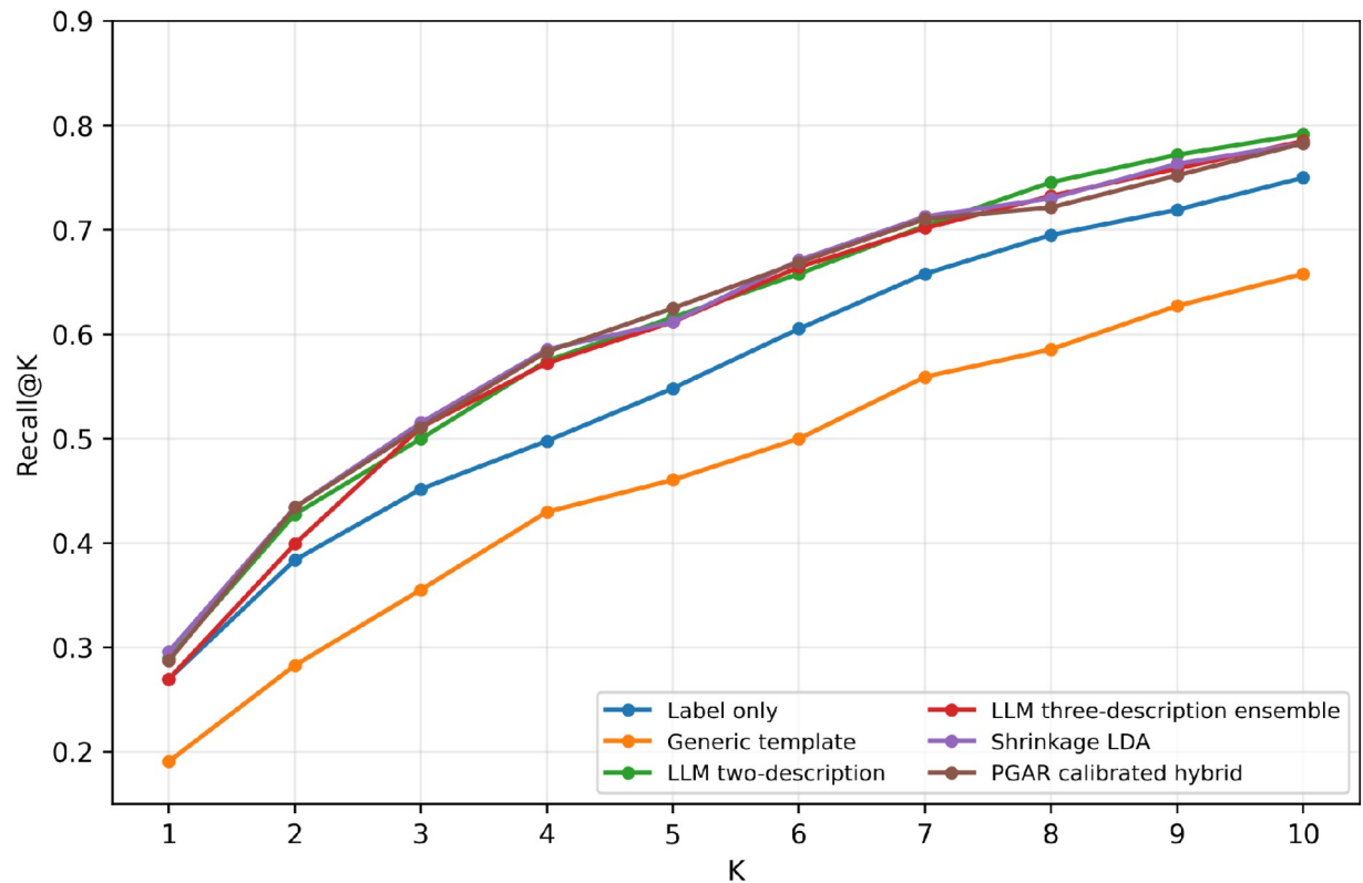
Figure 4. Recall@K curves for representative prompt, visual, and fused methods. Every point is calculated from the same 456 held-out predictions.
